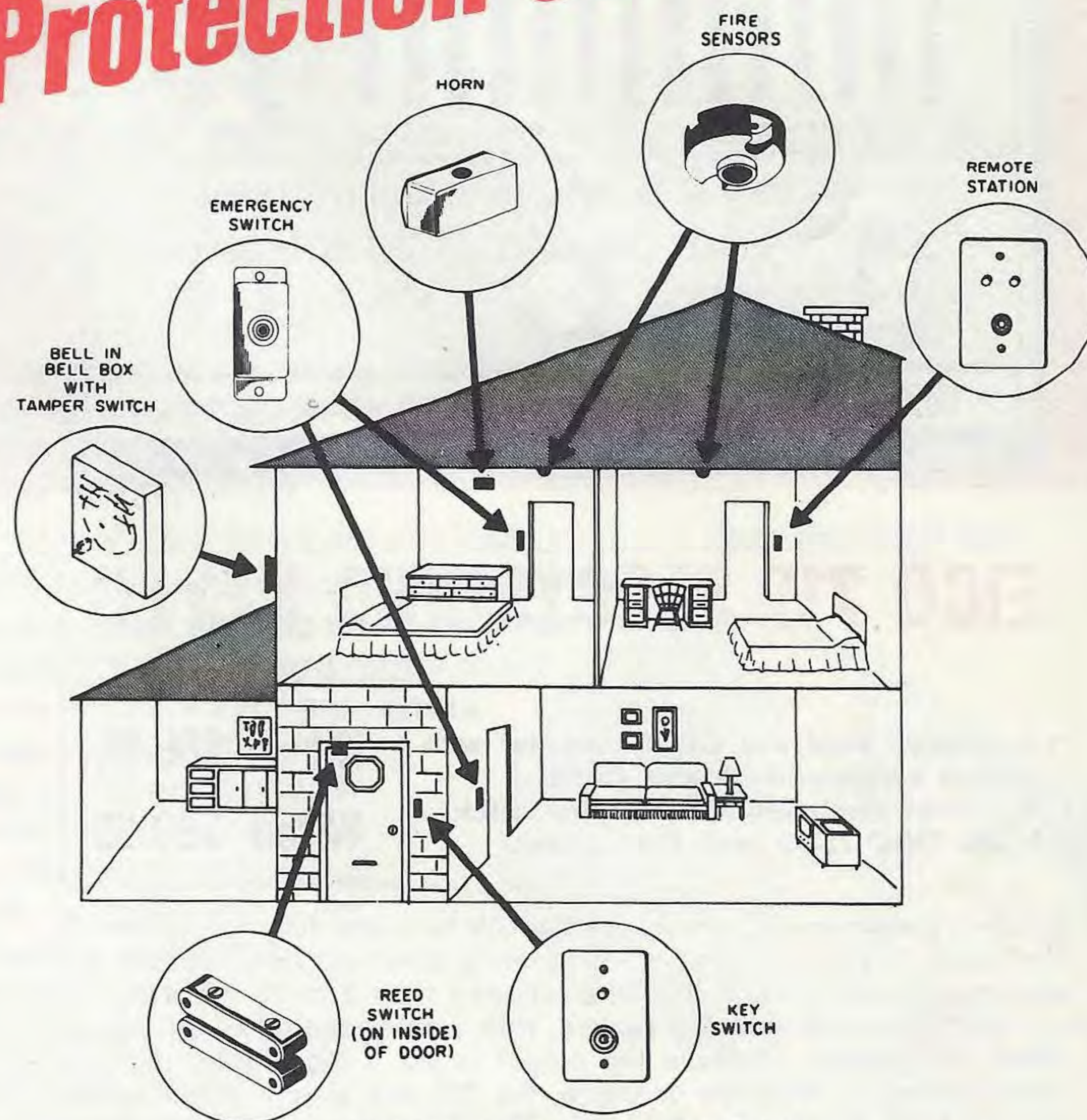
TYPICAL ALARM INSTALLATION
